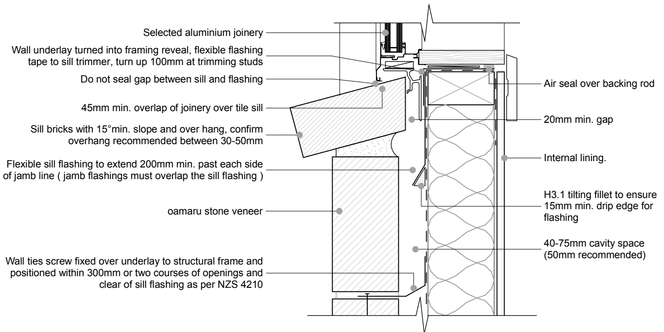
D-04 | OAMARU STONE-SILL DETAIL - | 1:5
