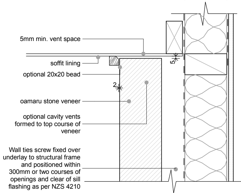
D-01 | OAMARU STONE -SOFFIT DETAIL - | 1:5
