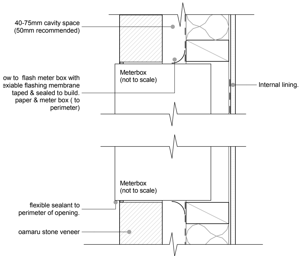
D-10 | OAMARU STONE -METER-BOX DETAIL - | 1:5
