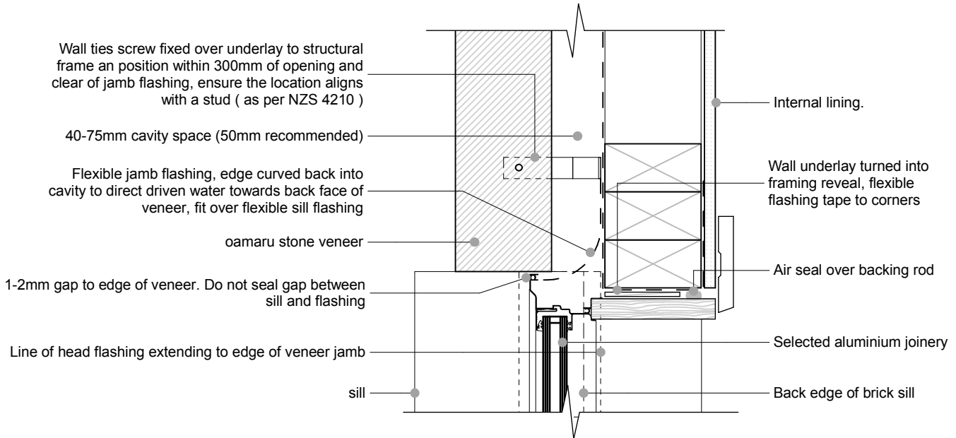
D-05 | OAMARU STONE-JAMB DETAIL - | 1:5
