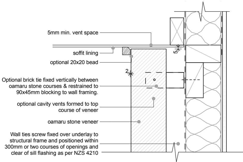
D-07 | OAMARU STONE -ALT. SOFFIT DETAIL - | 1:5
