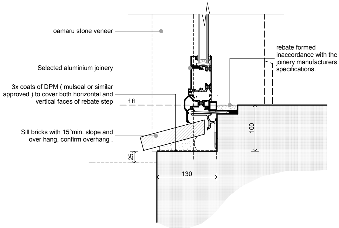
D-06 | OAMARU STONE-DOOR SILL DETAIL - | 1:5
