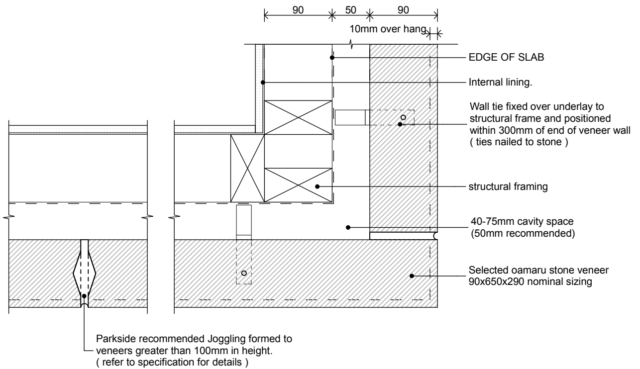
D-08 | OAMARU STONE-CORNER JUNCTION - | 1:5
