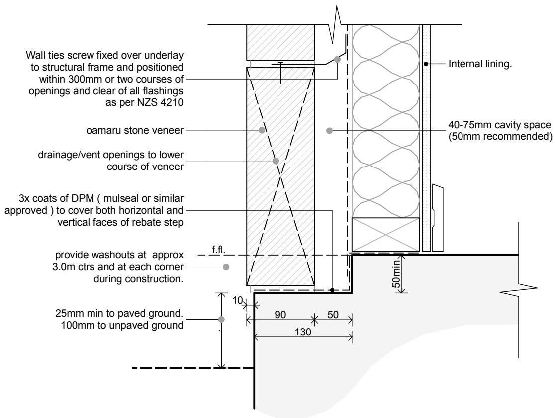
D-02 | OAMARU STONE -BASE DETAIL - | 1:5
