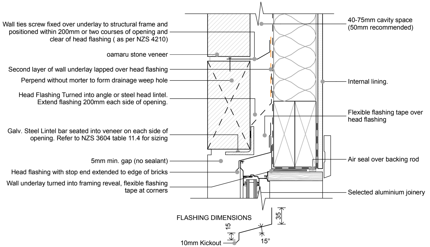
D-03 | OAMARU STONE-HEAD DETAIL - | 1:5
