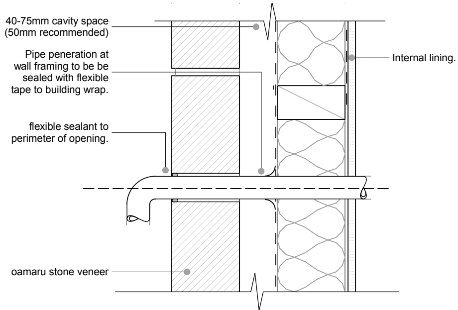
D-09 | OAMARU STONE -PENERATION DETAIL - | 1:5
